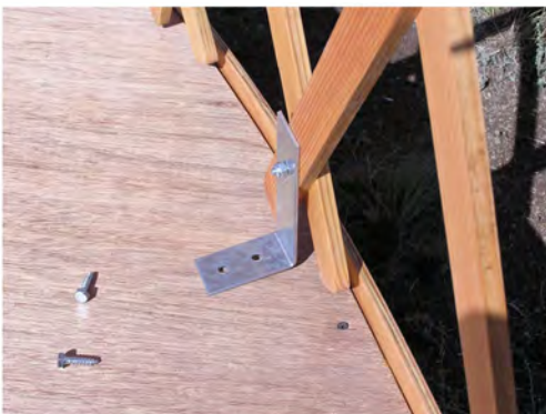
Steel brackets anchor lattice wall to deck.
